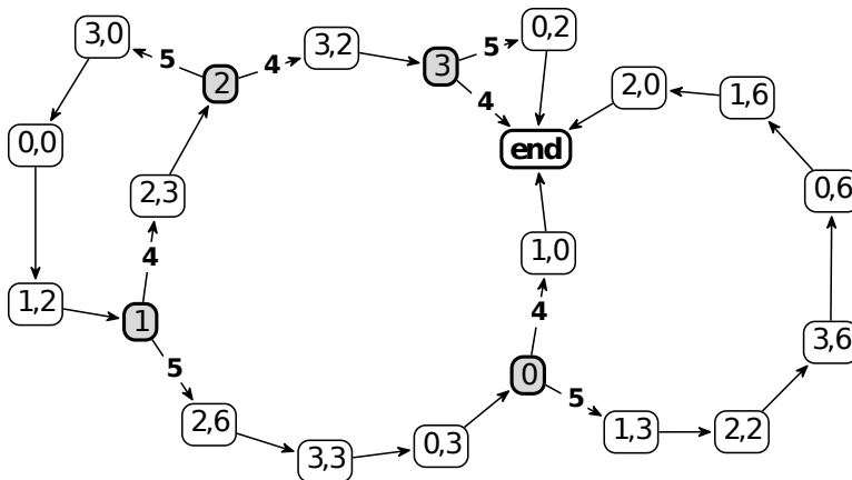
FIGURE 3. The graph in Figure 2 enlarged to include the branch-points, which are the shaded nodes. The unique infinite path follows the loop on the left of the graph.
