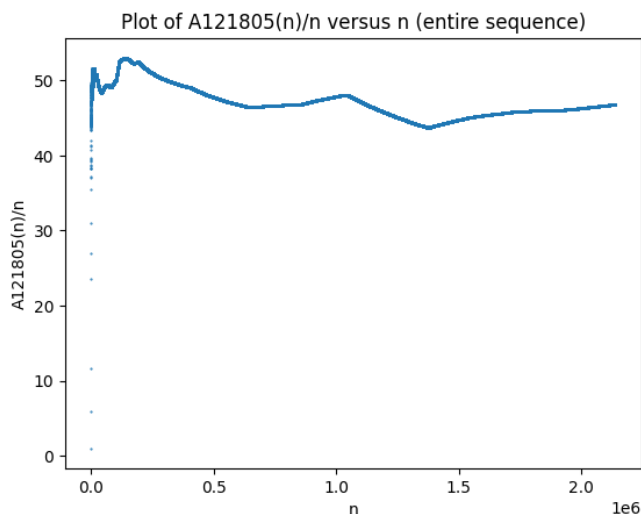
FIGURE 1. Plot of A121805(n)/n as n goes from 1 to 2137453. The final point has ordinate 46.78\dots
