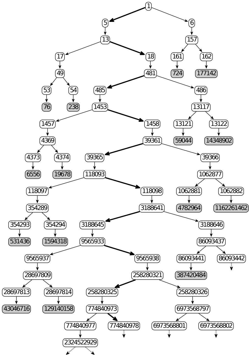
FIGURE 4. A portion of the base-3 child graph G_c . The thick lines are the start of the unique infinite path ( \underline{A367621} ). The shaded nodes are the landmines that must be avoided. Short vertical arrows represent long unbranched paths.
